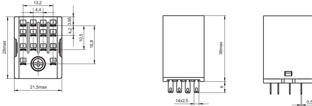
HF18FF-□/□□-4Z1□□□□
