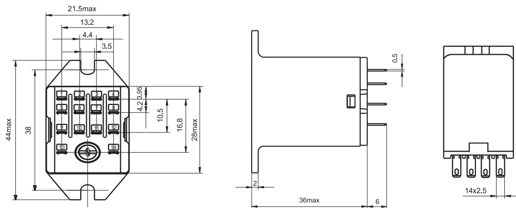
HF18FF-□/□□-4Z5□□□□
